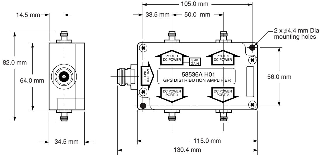
Figure 2. 58536A H01 GPS Distribution Amplifier
