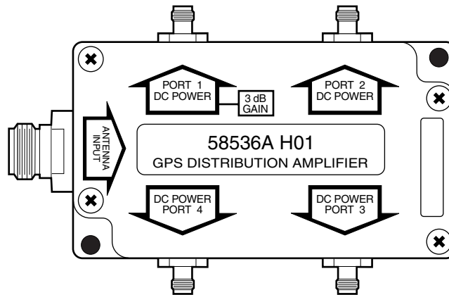
Figure 1. 58536A H01 GPS Distribution Amplifier
